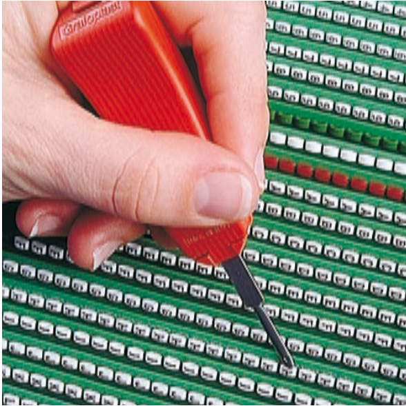
Step 1 Collect the marking elements on the applicator
